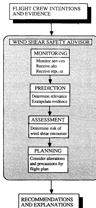
Fig. 2 Functions of the Wind Shear Safety Advisor.
